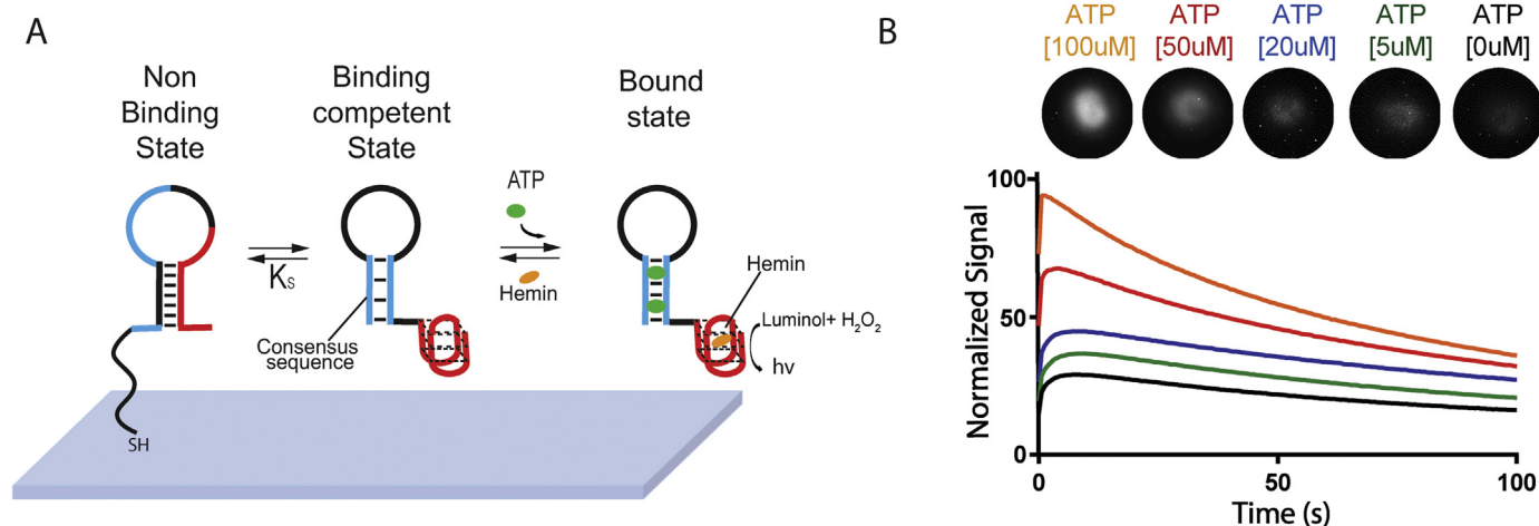
Fig. 4. : (A) ATP-regulated DNA-nanoswitches coexist in two mutually exclusive stem-loop conformations, i.e. “Non-Binding” and “Binding-competent”. The binding of ATP pushes this conformational equilibrium towards the “Bound” state, thus triggering the hemin/G-quadruplex structuring. (B) Chemiluminescence nanoswitch #3 spectra generated by the hemin/G-quadruplex aptamer ATP complex, in the presence of \text{H}_2\text{O}_2 /luminol and different concentrations of ATP. As the concentration of ATP is elevated, the chemiluminescence is intensified, consistent with the higher content of the assembled DNAzyme G-quadruplex structure.
